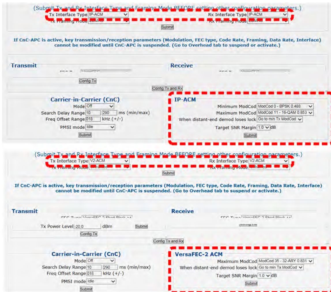
Figure 7-12. Configuration | Modem page (ACM Modes)
