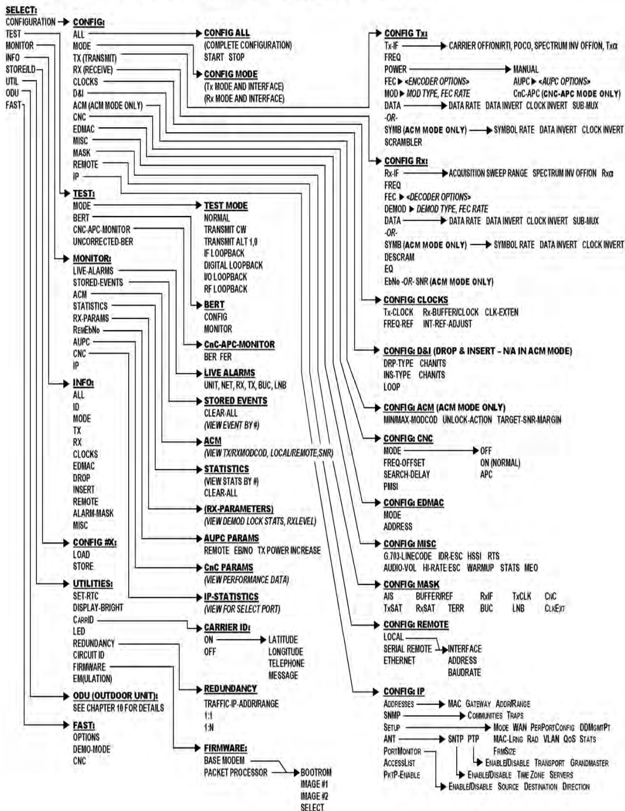
Figure 6-2. CDM-625A Principle Menu Tree (FW Ver. 1.4.1)
