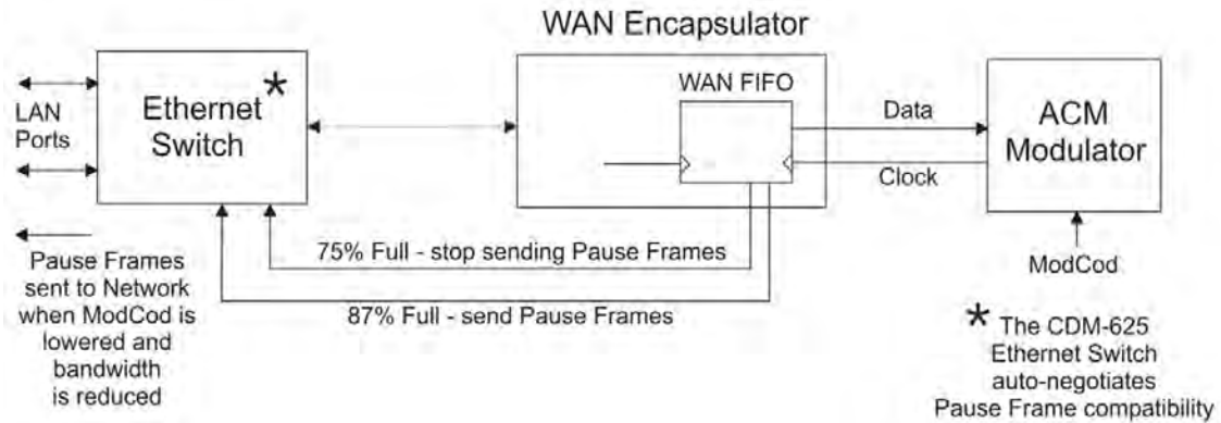
Figure M-5. CDM-625A – ACM Congestion Control
