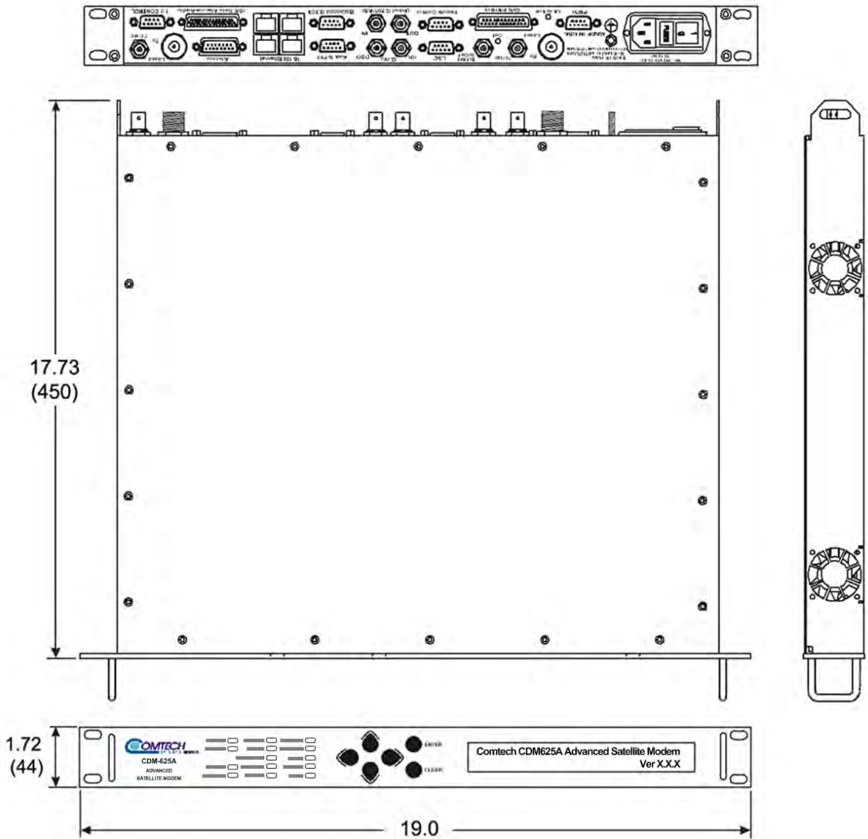
Figure 1-2. CDM-625A Dimensional Envelope
